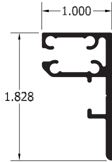
FRONT LOAD SOFT SIGNAGE TENSION FRAME #3092
